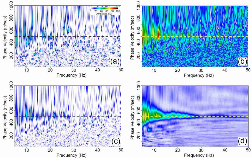
Figure 6. Dispersion images obtained from the record in Figure 5a by using (a) a scheme by Park et al. (2004), (b) the conventional wavenumber ( K_x-K_y ) approach incorporated into the active scheme by Park et al. (1998), (c) the method presented in this paper, and (d) the scheme used for (c) with incorporation of broad-band summation (BBS) scheme.
