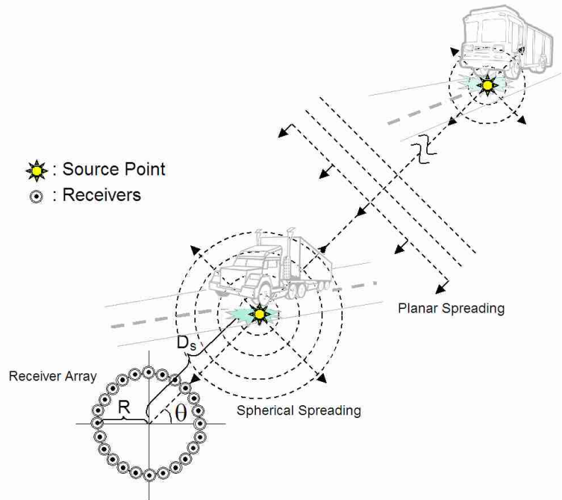
Figure 1. Schematic showing spherical and planar propagation of surface waves generated at relatively close and distant locations, respectively.
