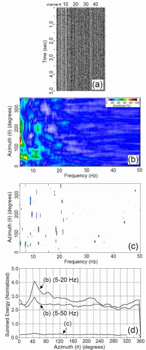
Figure 5. (a) Synthetic record in Figure 2a with random noise added, corresponding images of azimuth energy distribution obtained from the scheme by Park et al. (2004) (b) with and (c) without incorporation of BBS scheme, and (d) curves obtained by summing energy in (b) and (c).
