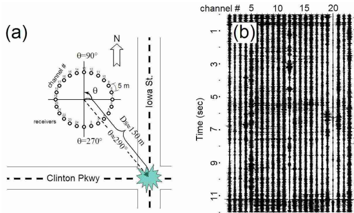
Figure 7. (a) Field map showing relative location of the receiver array and major point of surface wave generation during the survey at the University of Kansas soccer field, Lawrence, Kansas, and (b) a 12-sec long field record obtained from this survey.
