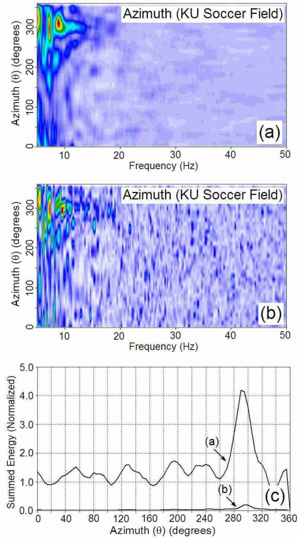
Figure 9. Images of azimuth energy distribution obtained from the field record of Figure 7b by using the scheme in Park et al. (2004) (a) with and (b) without incorporation of broad-band summation (BBS) scheme, and (c) curves obtained by summing energy in (a) and (b) along the frequency axis.
