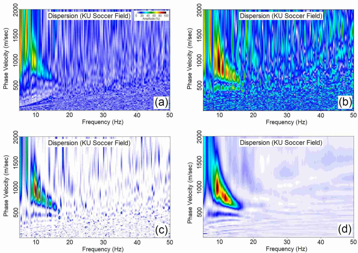
Figure 8. Dispersion images obtained from the field record of Figure 7b by using (a) a scheme by Park et al. (2004), (b) the conventional wavenumber ( K_x - K_y ) approach incorporated into the active scheme by Park et al. (1998), (c) the method presented in this paper, and (d) the scheme used for (c) with incorporation of broad-band summation (BBS) scheme.
