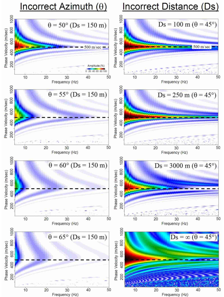
Figure 3. Dispersion images obtained from the synthetic record in Figure 2a by using an active processing scheme with incorrect azimuth (left column) and source distance (right column).
