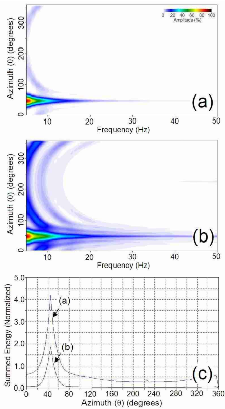
Figure 4. Images of azimuth energy distribution obtained from the record in Figure 1a (a) by using a scheme by Park et al. (2004) alone, (b) with an addition of another enhancement scheme of broad-band summation (BBS), (c) curves obtained by summing all the energy in (a) and (b).
